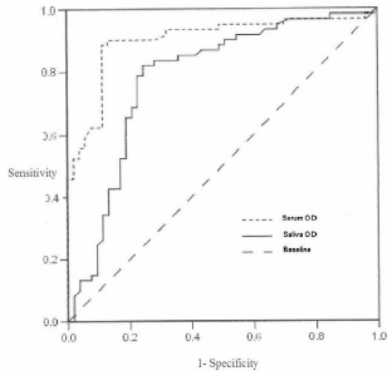
Figure 3. The ROC curve of ELISA test for serum and saliva anti- H. pylori IgG
